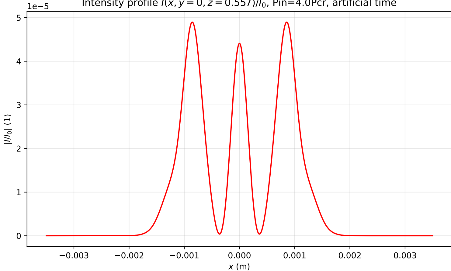
Intensity profile I(x, y = 0, z = 0.557)/I_0 , P_{in}=4.0P_{cr} , artificial time
